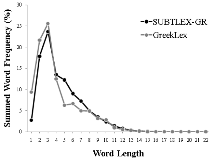
Figure 1. Distribution of the percentages of summed word frequency as a function of word length (measured in number of letters) for the GreekLex and the SUBTLEX-GR entries.
